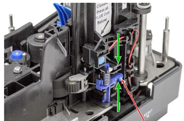
Pinch the tab on the Latch to open
